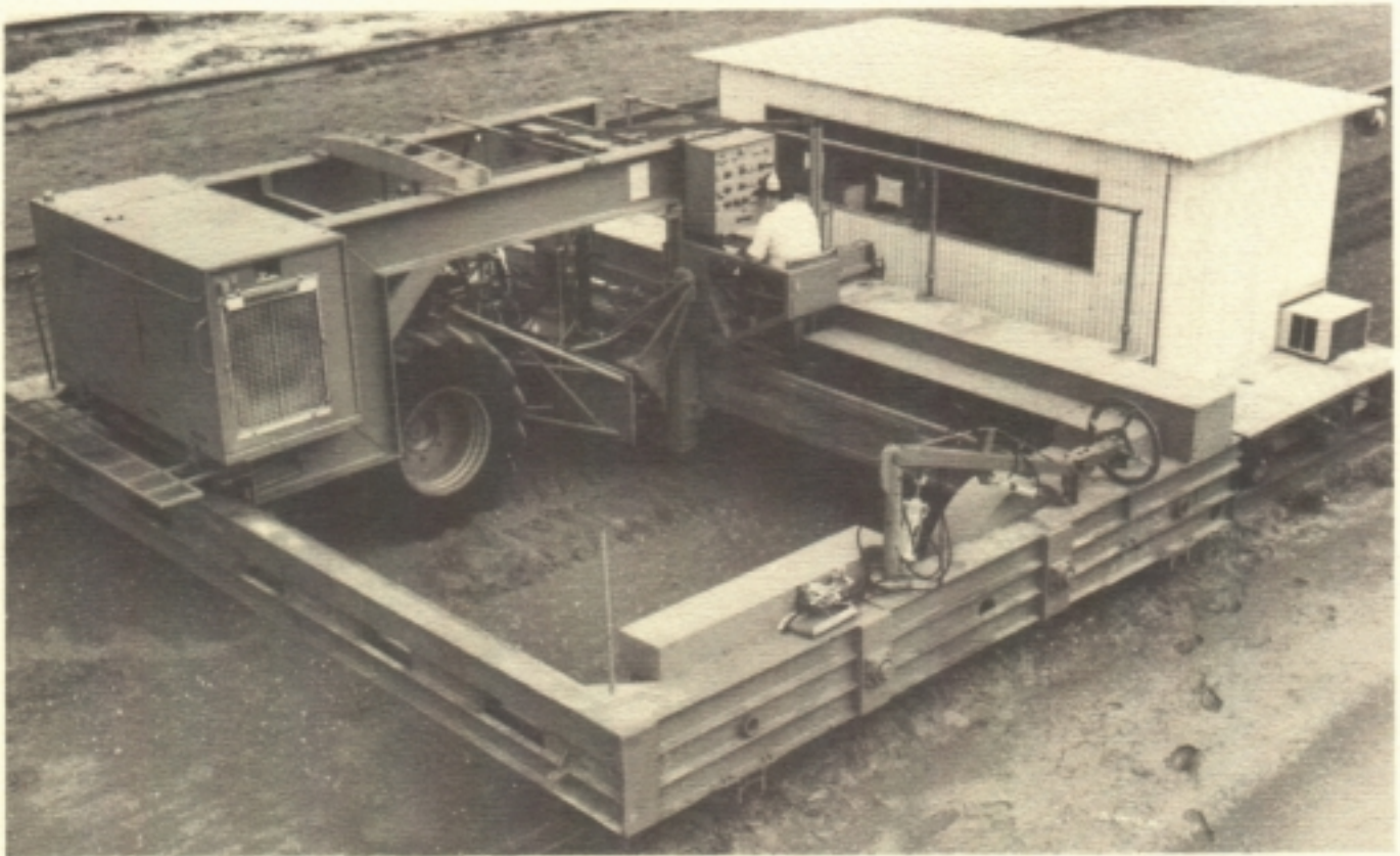
The NSDL single wheel research machine used to study the soil and tire parameters influencing traction and mobility.
