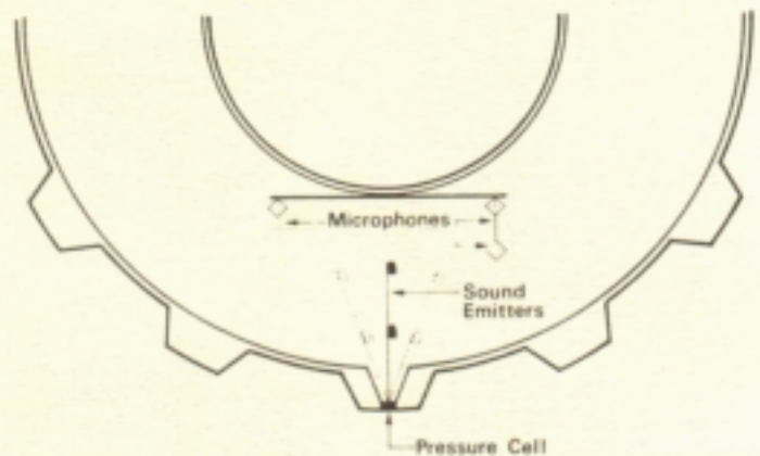
Tangential and normal stresses and deformations of pneumatic tires are measured with stress cells and a sonic digitizing unit.
