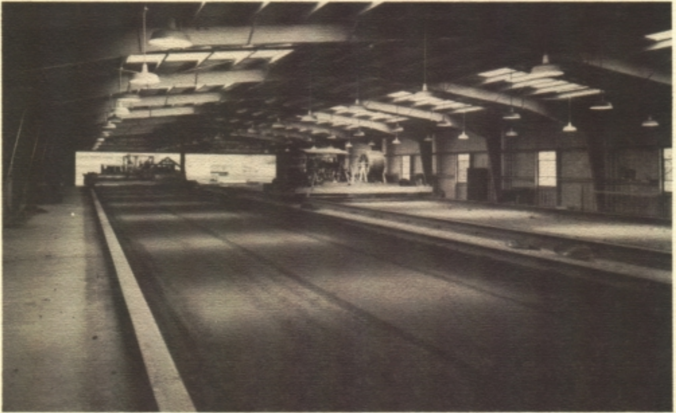
Two covered soil bins 57.3 m (190-feet) long, 6.1 m (20-feet) wide, and 1.8 m (six-feet) deep provide environmental control for conducting complex soil-machine research measurements year around.
