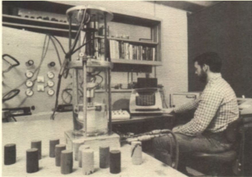
Research apparatus to develop soil compaction models.
